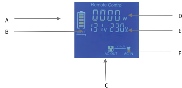
DISPLAY AFSTANDBEDIENING TRANSFERSWITCH MODE (1000W / 1500W / 2000W / 3000W)
