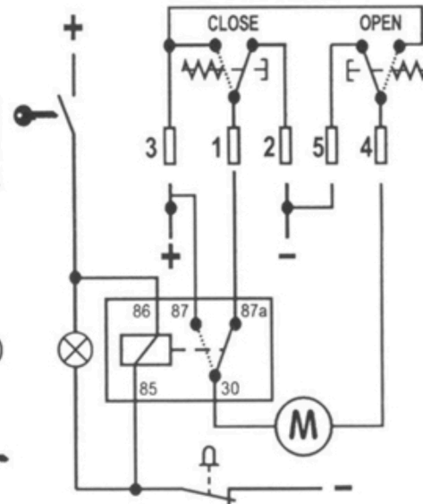
AUTOMATIC STEP RETRACT
