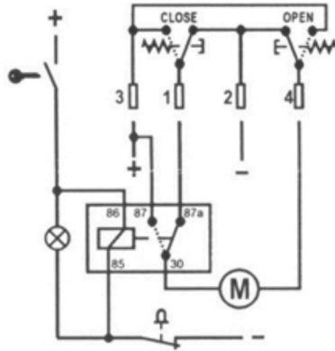
AUTOMATIC STEP RETRACT
