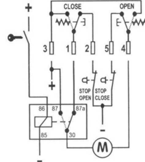
AUTOMATIC STEP RETRACT WITH 2 STOP SWITCHES
