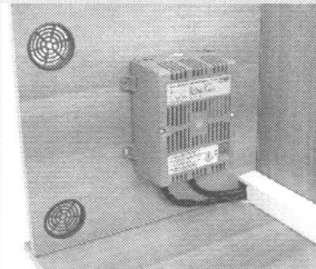
Fig.2 - VERTICAL INSTALLATION
