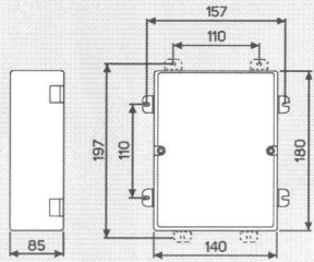
Fig.1 - DIMENSIONS (mm):
